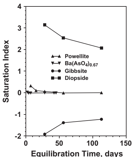
FIGURE 6.1 Saturation indices ( SI = \log IAP - \log K_{sp} ) for gibbsite [ Al(OH)_3 ] and diopside [ CaMg(SiO_3)_2 ] in a spent oil shale leachate tend toward zero with equilibration time, but solution IAP values are one to two orders of magnitude removed from the respective K_{sp} values after 130 days (Essington and Spackman, 1988). Powellite [ CaMoO_4 ] and Ba(AsO_4)_{0.67}(c) saturation indices rapidly approach zero in constant ionic strength background electrolyte solutions (Essington, 1988a; 1990).
