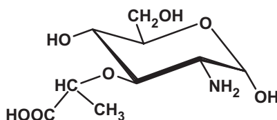
FIGURE 4.8 Amino sugars that are commonly observed in soil.
