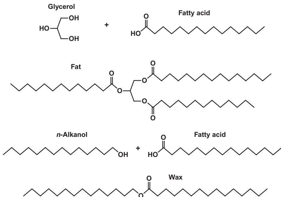
FIGURE 4.16 Fats are esters of glycerol and fatty acids; whereas, waxes are esters of an n -alcohol and a fatty acid. The fatty acids in this figure are saturated, because all bonds in the alkyl carbon chain are single bonds.
