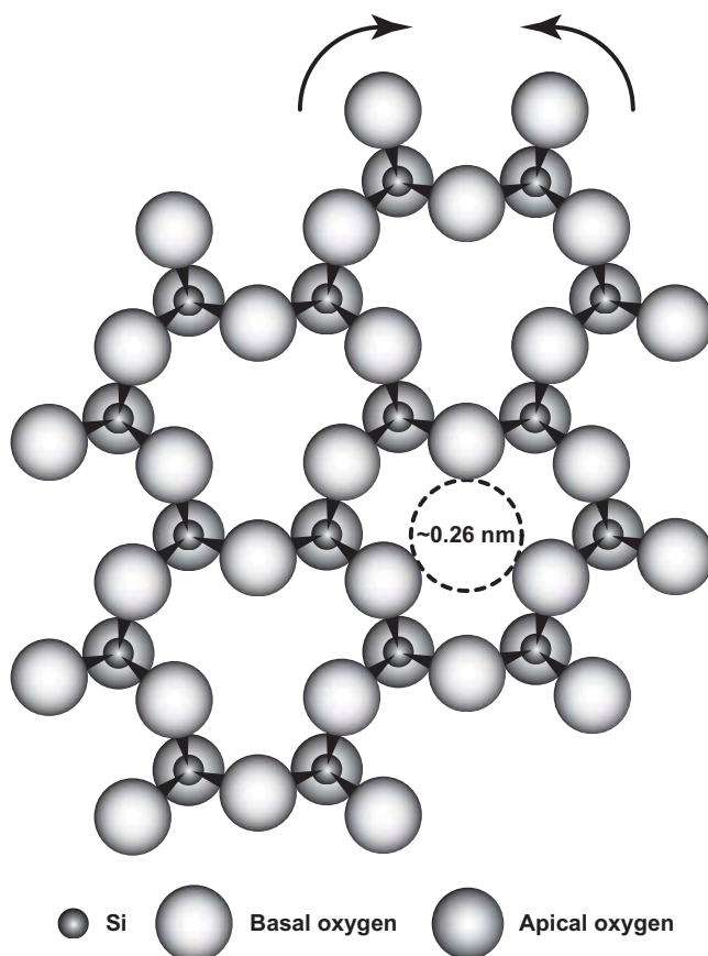
FIGURE 7.2 Schematic of the siloxane ditrigonal cavity on the planar surface of a phyllosilicate. The rotation of the silica tetrahedral about the Si-apical oxygen axis (in the directions of the arrows) distorts the ideal hexagonal configuration, resulting in the ditrigonal arrangement of the silica tetrahedra and a cavity diameter of \sim 0.26 nm.
