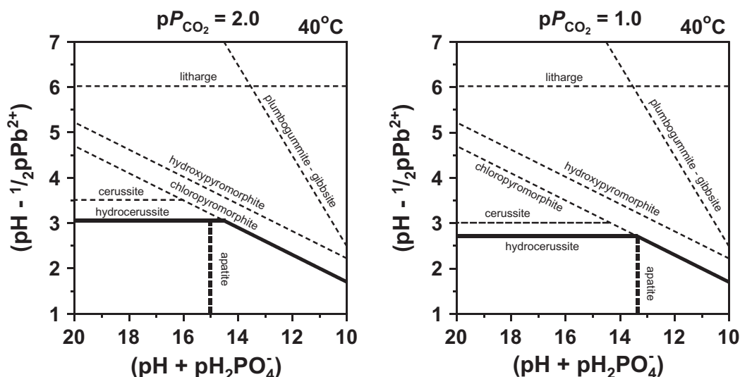
FIGURE 6.14 Activity ratio diagrams illustrating the stability of lead carbonates and lead phosphates at 40°C and 0.101 MPa as a function of solution pH, \text{H}_2\text{PO}_4^- activity, and \text{CO}_2 partial pressure. Mineral and liquid water activities are unity. The controlling conditions and the chemical formula that correspond to the mineral names are given in the legend to Figure 6.12.
