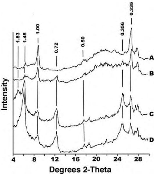
FIGURE 2.44 X-ray diffractograms of the clay fraction of a Delhi soil. (a) K^+ - saturated, 600°C; (b) K^+ - saturated, 25°C; (c) Mg^{2+} - and glycerol-saturated; (d) Mg^{2+} -saturated. Peaks are identified by d-spacing (in nm).
