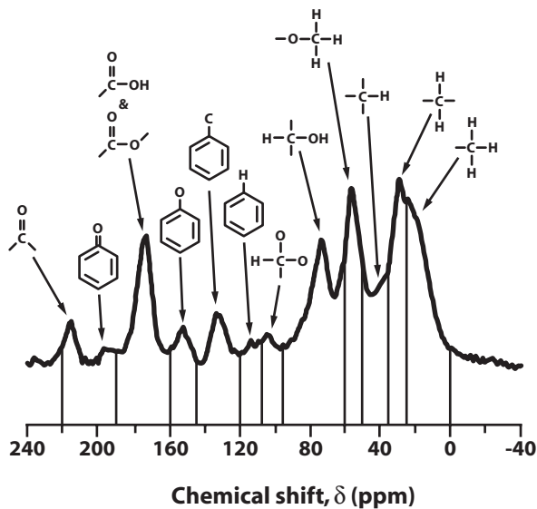
FIGURE 4.27 Example of a cross-polarization, magic angle spinning 13 C nuclear magnetic resonance (CPMAS 13 C NMR) spectra of humic acid from Conte et al. (1997). The vertical lines delineate the typical chemical shift assignments (from Table 4.6).
