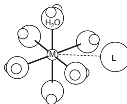
Outer-Sphere Complex
