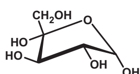
D-xylose
