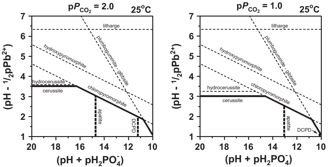
FIGURE 6.12 Activity ratio diagrams illustrating the stability of lead carbonates and lead phosphates at 25°C and 0.101 MPa as a function of solution pH, \text{H}_2\text{PO}_4^- activity, and \text{CO}_2 partial pressure. Controlling conditions are (\text{pH} + \text{pCl}^-) = 11.3 , (\text{pH} - \frac{1}{2} \text{pCa}^{2+}) controlled by calcite, and (\text{pH} - \frac{1}{3} \text{pAl}^{3+}) controlled by gibbsite. Mineral and liquid water activities are unity. Litharge, \text{PbO} ; cerussite, \text{PbCO}_3 ; hydrocerussite, \text{Pb}_3(\text{CO}_3)_2(\text{OH})_2 ; hydroxypyromorphite, \text{Pb}_5(\text{PO}_4)_3\text{OH} ; chloropyromorphite, \text{Pb}_5(\text{PO}_4)_3\text{Cl} ; plumbogummite, \text{PbAl}_3(\text{PO}_4)_2(\text{OH})_5 \cdot \text{H}_2\text{O} ; apatite, \text{Ca}_5(\text{PO}_4)_3\text{OH} ; dicalcium phosphate dihydrate (DCPD), \text{CaHPO}_4 \cdot 2\text{H}_2\text{O} .
