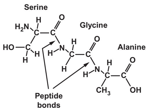
FIGURE 4.11 A peptide composed of the amino acids serine, glycine, and alanine. The individual amino acid monomers in peptides and proteins are linked through peptide bonds.
