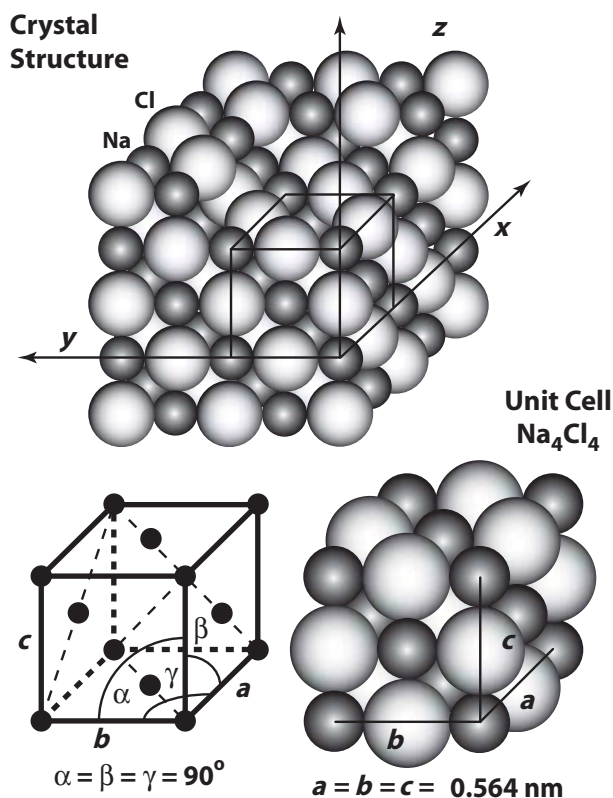
FIGURE 2.7 The halite (NaCl) lattice and unit cell.
