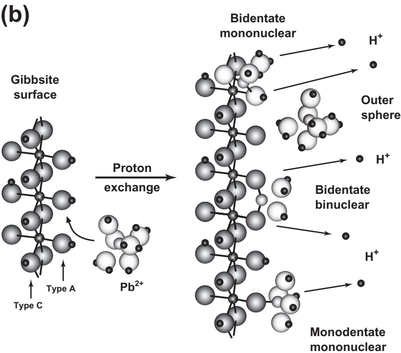
FIGURE 7.5 (continued).
