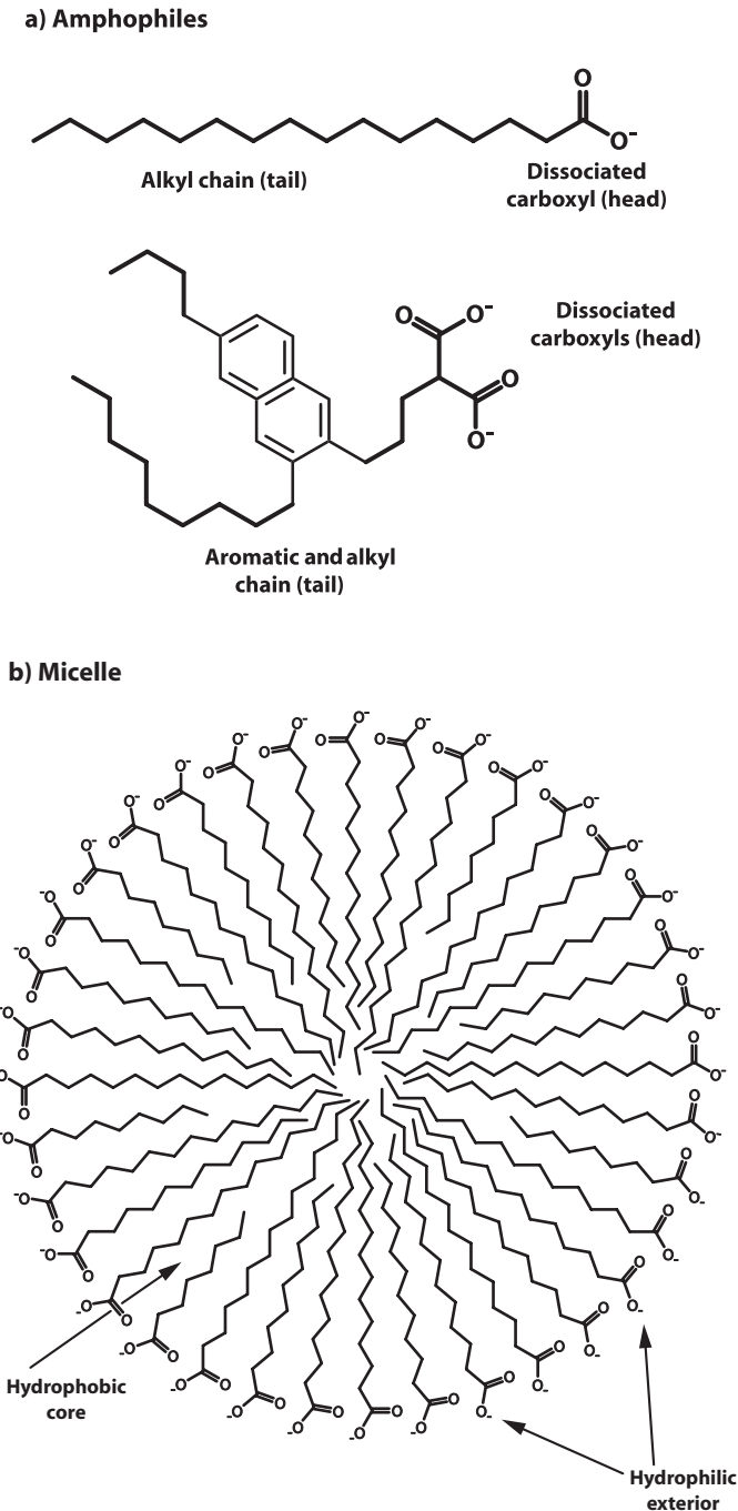
FIGURE 4.25 The self-aggregation theory of humic substance production is based on the premise that biopolymer degradation products are amphiphilic, consisting of hydrophilic (polar or ionic) and hydrophobic molecular segments (a). In solution, the degradation byproducts form micelle-like structures (b), composed of a hydrophilic outer layer and a hydrophobic core. Accumulation of humic substances on soil surfaces (c) is initiated by the reaction of hydrophilic moieties with surface oxygens (electrostatic interactions) or surface metal cations (direct ionic/covalent bonds). The hydrophobic portions of these surface molecules are shielded from the polar aqueous phase by a second layer of amphiphiles to form a bilayer.
