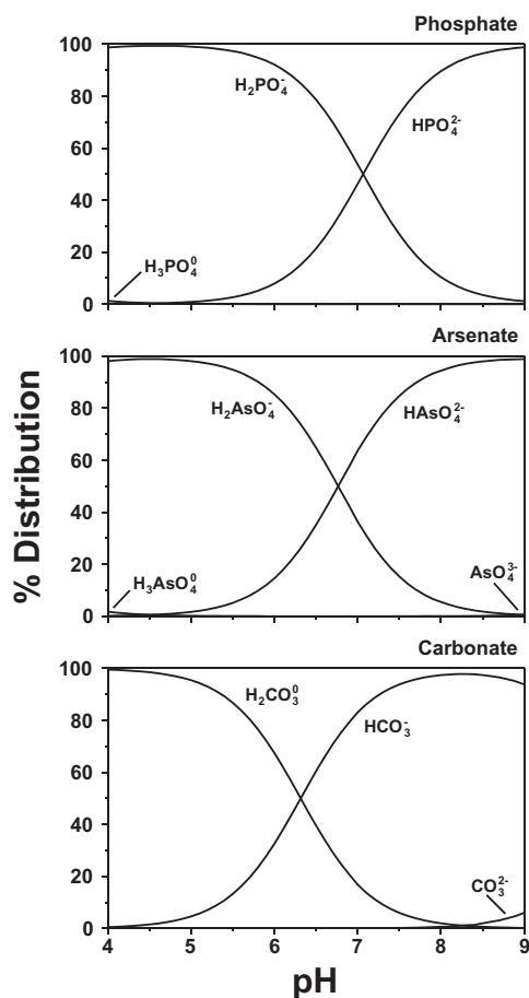
FIGURE 5.7 The distribution of weak Lowry-Brønsted acids as a function of solution pH at 25°C. The diagrams were constructed using total concentrations of: 10^{-5} M for \text{PO}_4 , 10^{-6} M for \text{AsO}_4 , 10^{-3} M for \text{CO}_3 , and a background electrolyte of 10^{-2} M for \text{NaClO}_4 . The \text{p}K_a values employed to construct the diagrams were obtained from Table 5.8.
