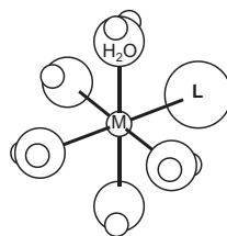
Inner-Sphere Complex
