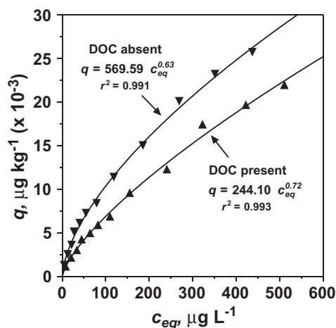
FIGURE 7.25 The adsorption of fluridone by DOC- and \text{Ca}^{2+} -saturated STx-1 montmorillonite in the presence and absence of 100 \text{ mg L}^{-1} DOC. The experimental data are indicated by the closed triangles. The Freundlich adsorption isotherm models, represented by the lines and corresponding equations, were generated by nonlinear least-squares regression analysis. The adsorption data were obtained by equilibrating 0.3-g samples of DOC- and \text{Ca}^{2+} -saturated clay and 30 mL of 10 \text{ mM} \text{CaCl}_2 containing varied concentrations of the herbicide. The DOC was extracted from a Lexington silt loam (Ultic Hapludalf) surface soil. The suspensions were equilibrated for 24 h at 20^\circ\text{C} .
