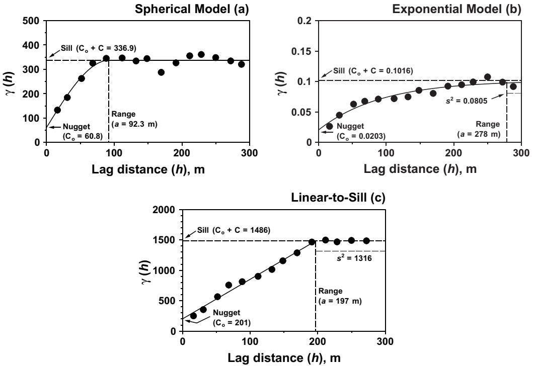
FIGURE 1.7 Examples of variograms and commonly applied semivariogram models: (a) ECEC ( \text{mmol}_c \text{ kg}^{-1} ), spherical model; (b) \ln \text{ ex-Mn} ( \text{mg kg}^{-1} ), exponential model; and (c) \text{ex-K} ( \text{mg kg}^{-1} ), linear-to-sill model.
