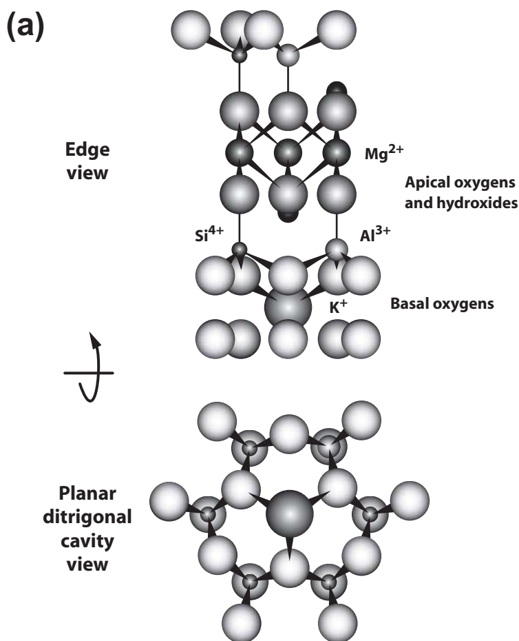
FIGURE 7.7 Example of inner-sphere complexation of K^{+} by trioctahedral vermiculite (a) as seen from side and planar views of the siloxane ditrigonal cavity. The K^{+} ion is bound in octahedral coordination by three basal oxygen atoms of one silica sheet and by three in the opposing sheet. An example of an outer-sphere complexation of a hydrated cation, such as Ca^{2+} , is shown with montmorillonite (b).
