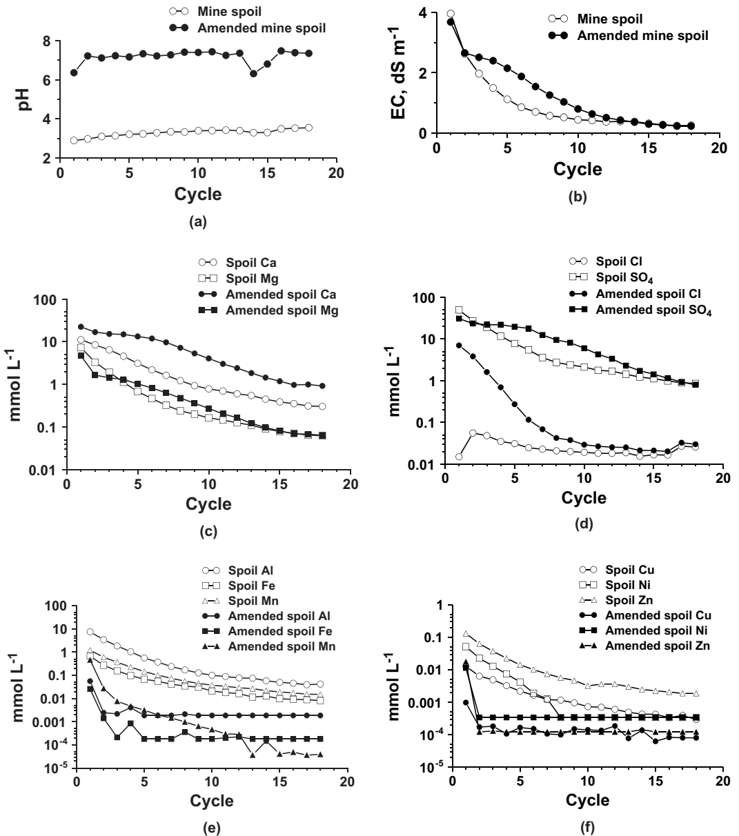
FIGURE 10.6 The chemical characteristics of leachates as a function of weathering cycle from a laboratory study of simulated weathering used to evaluate the potential long-term effectiveness of using lime-stabilized sewage sludge to neutralize acidity generated by a pyritic mine spoil: (a) pH, (b) electrical conductivity (EC), (c) Ca and Mg, (d) Cl and SO 4 , (e) Al, Fe, and Mn, and (f) Cu, Ni, and Zn. (Modified from Abbott, D.E., M.E. Essington, M.D. Mullen, and J.T. Ammons. Fly ash and lime-stabilized sewage sludge mixtures in mine spoil reclamation: simulated weathering. J. Environ. Qual. 30:608–616, 2001.)
