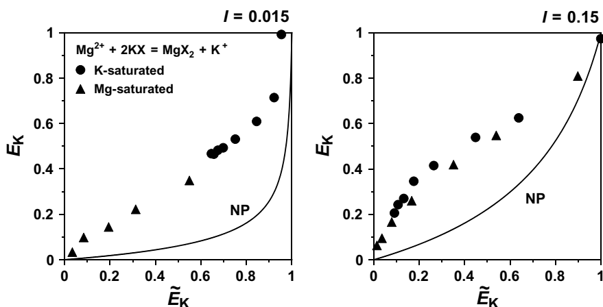
FIGURE 8.11 Exchange isotherms for binary KX-MgX 2 exchange in Loring (Oxyaquic Fragiudalf) soil as a function of ionic strength (0.015 and 0.15). The nonpreference isotherms (NP) were computed using Equation 8.75.
