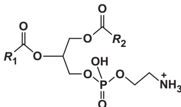
FIGURE 4.14 The two common phospholipids in soil are phosphatidylcholine and phosphatidylethanolamine. These compounds are esters of glycerol (1,2,3-propantriol) and long-chain alkanolic acids (fatty acids) and phosphate ( R_1 and R_2 represent the alkyl chains).
