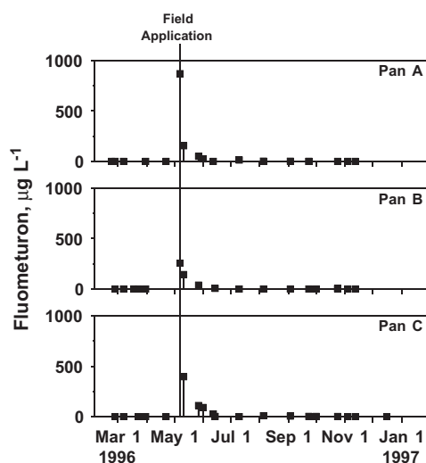
FIGURE 5.19 The concentration of the herbicide fluometuron collected by three tension-free pan lysimeters. The pans are located within a 1-acre production cotton field at Ames Plantation (near La Grange, TN) and emplaced at a depth of 90 cm. Field application of the herbicide occurred on May 6, 1996; whereupon rapid leaching of the herbicide is observed during a rainfall event.
