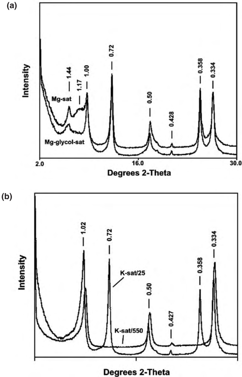
FIGURE 2.42 X-ray diffractograms of clay-sized materials separated from an abandoned mine spoil material: (a) \text{Mg}^{2+} - and \text{Mg}^{2+} glycol-saturated and (b) \text{K}^{+} -saturated (25 and 550°C). Peaks are identified by d-spacing (in nm).
