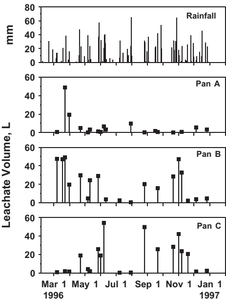
FIGURE 5.18 The variability in leachate collection by three tension-free pan lysimeters. The pans are located within a 1-acre production cotton field at Ames Plantation (near La Grange, TN) and emplaced at a depth of 90 cm. Rainfall data are collected on-site.
