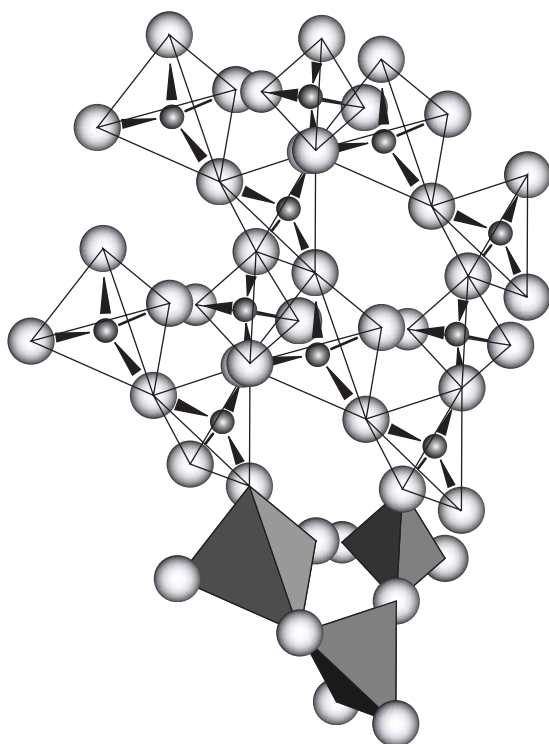
FIGURE 2.16 The tectosilicate framework structure of quartz [ \text{SiO}_2 ]. The dark circles represent Si atoms and the light circles are oxygen atoms.
