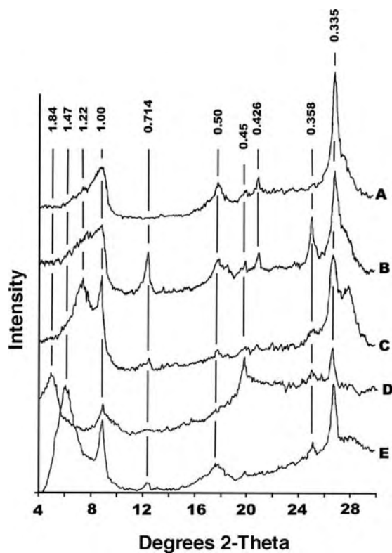
FIGURE 2.43 X-ray diffractograms of the clay fraction of a San Emigdio soil. (a) \text{K}^+ -saturated, 550^\circ\text{C} ; (b) \text{K}^+ -saturated, 300^\circ\text{C} ; (c) \text{K}^+ -saturated, 25^\circ\text{C} ; (d) \text{Mg}^{2+} - and glycerol-saturated; (e) \text{Mg}^{2+} -saturated. Peaks are identified by d-spacing (in nm).
