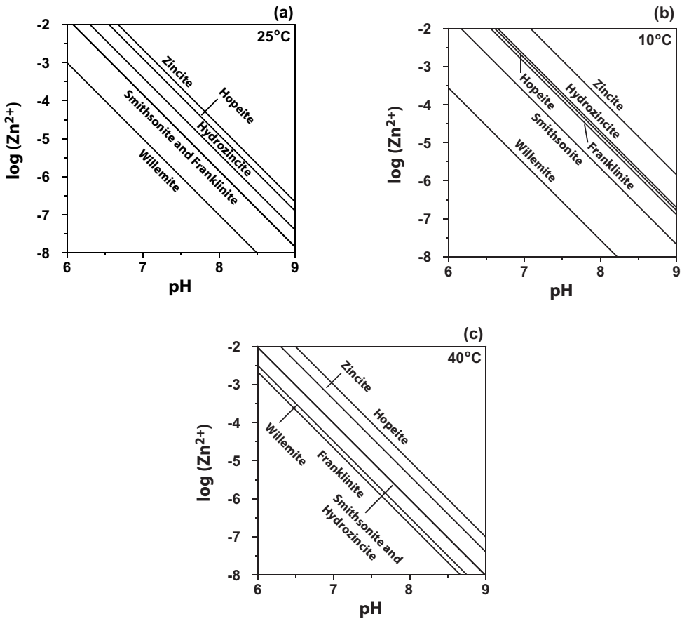
FIGURE 6.9 Stability of the Zn-bearing minerals, zincite [ \text{ZnO} ], smithsonite [ \text{ZnCO}_3 ], hydrozincite [ \text{Zn}_5(\text{OH})_6(\text{CO}_3)_2 ], hopeite [ \text{Zn}_3(\text{PO}_4)_2 \cdot 4\text{H}_2\text{O} ], franklinite [ \text{ZnFe}_2\text{O}_4 ], and willemite [ \text{Zn}_2\text{SiO}_4 ] as a function of solution pH and temperature: (a) 25°C, (b) 10°C, and (c) 40°C. The following conditions apply: 0.101 MPa pressure, solid and water activities are unity, \text{CO}_2 partial pressure is 10^{-2} , solution activity of \text{H}_2\text{PO}_4^- is controlled by hydroxyapatite and calcite, \text{H}_4\text{SiO}_4^0 activity is controlled by \text{H}_4\text{SiO}_4(\text{am}) , and \text{Fe}^{3+} is controlled by goethite [ \text{FeOOH} ].
