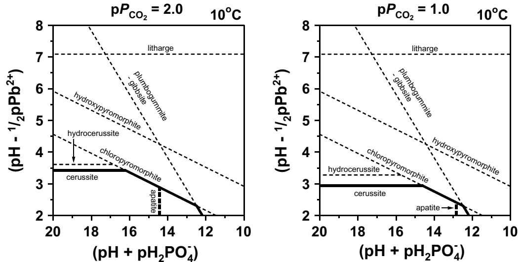
FIGURE 6.13 Activity ratio diagrams illustrating the stability of lead carbonates and lead phosphates at 10°C and 0.101 MPa as a function of solution pH, \text{H}_2\text{PO}_4^- activity, and \text{CO}_2 partial pressure. Mineral and liquid water activities are unity. The controlling conditions and the chemical formula that correspond to the mineral names are given in the legend to Figure 6.12.
