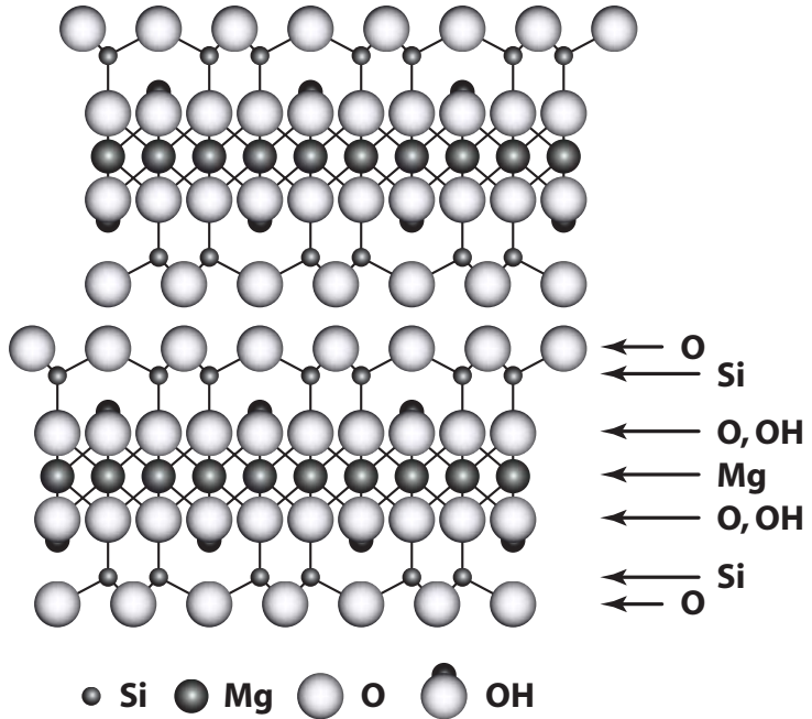
FIGURE 2.27 The structure of talc [Mg_3Si_4O_{10}(OH)_2] .
