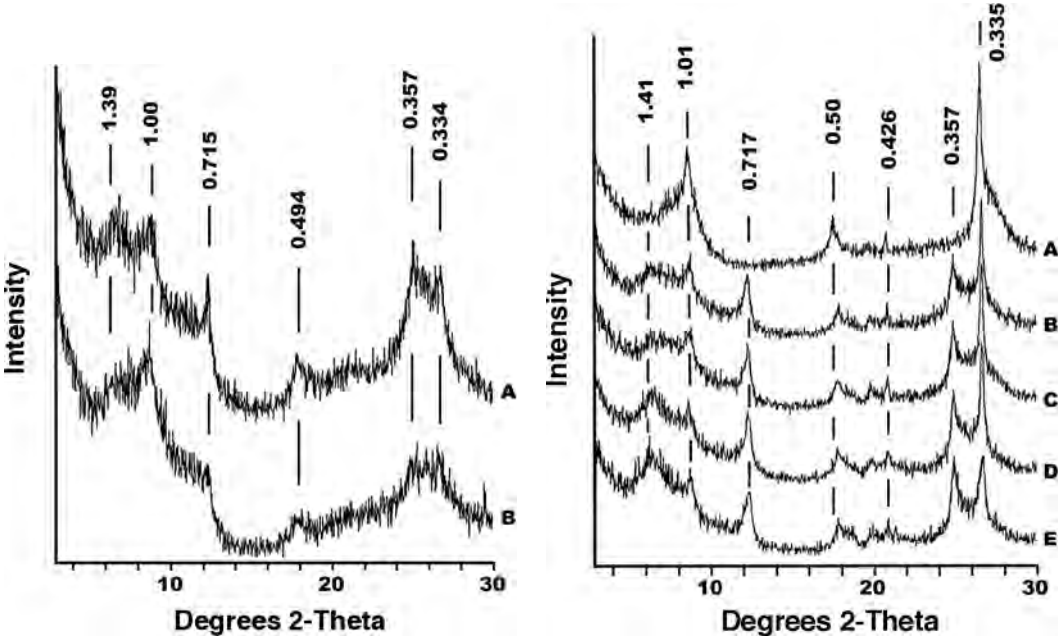
FIGURE 2.45 X-ray diffractograms of the clay fraction of a Loring soil. (a) Mg^{2+} - and glycol-saturated (A) and Mg^{2+} -saturated (B); (b) K^+ - saturated, 550°C (A), K^+ - and glycerol-saturated (B), K^+ - saturated, 300°C (C), K^+ saturated, 105°C (D), and K^+ - saturated, 25°C (E). Peaks are identified by d-spacing (in nm).
