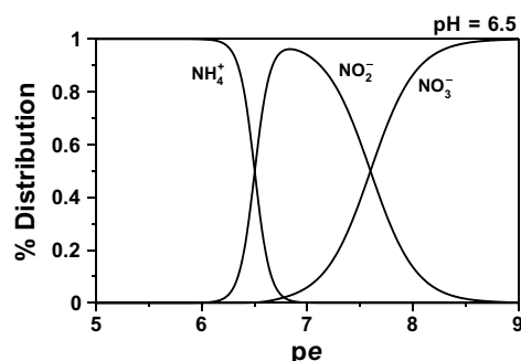
FIGURE 9.3 The predicted distribution of nitrogen as a function of pe in a pH 6.5 solution. The thermodynamic data in Table 9.1 were used to construct the figure.
