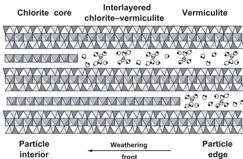
FIGURE 3.6 The alteration of chlorite occurs through a combined layer and edge weathering mechanism. Beginning at the particle edge, acidic conditions promote the dissolution of the hydroxy interlayer and the intrusion of layer charge-satisfying hydrated cations. The loss of octahedral cations in response to \text{Fe}^{\text{II}} oxidation and the reduction in layer charge by \text{Si}^{4+} substitution for tetrahedral \text{Al}^{3+} stabilizes alternating interlayers and results in an interstratified chlorite-vermiculite. As the layer weathering front proceeds into the particle interior, adjacent hydroxy-interlayers are dissolved at the particle edge and replaced by hydrated cations. The process continues into the chlorite core, until the hydroxyl-interlayers are dissolved and the transformation to the expansive vermiculite is complete.
