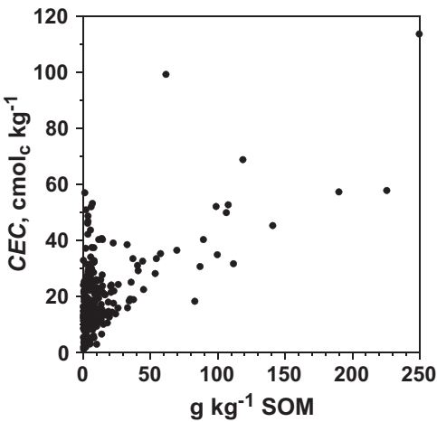
FIGURE 8.1 The cation exchange capacity ( CEC ) of 249 surface soil samples collected from around the U.S. as a function of soil organic matter content (SOM). Data were obtained from Batjes (1995).
