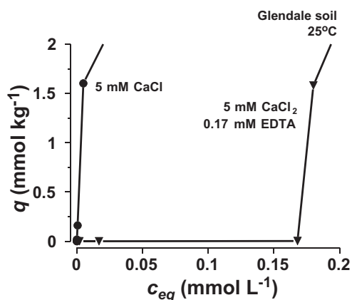
FIGURE 7.14 Adsorption isotherms characterizing the retention of nickel (Ni) by surface horizon (0 to 15 cm) samples of a Glendale soil (Typic Torrifluent) from 5 mM CaCl 2 (H-type isotherm) and 5 mM CaCl 2 + 0.17 mM EDTA (S-type isotherm) solutions. The adsorption data were obtained by equilibrating 11-g samples of soil and 11 mL of 5 mM CaCl 2 solutions containing varied concentrations of NiCl 2 . The suspensions were equilibrated for 24 h at 20 to 25°C. (Modified from Bowman, R.S., M.E. Essington, and G.A. O'Connor. Soil sorption of nickel: influence of solution composition. Soil Sci. Soc. Am. J. 45:860–865, 1981.)
