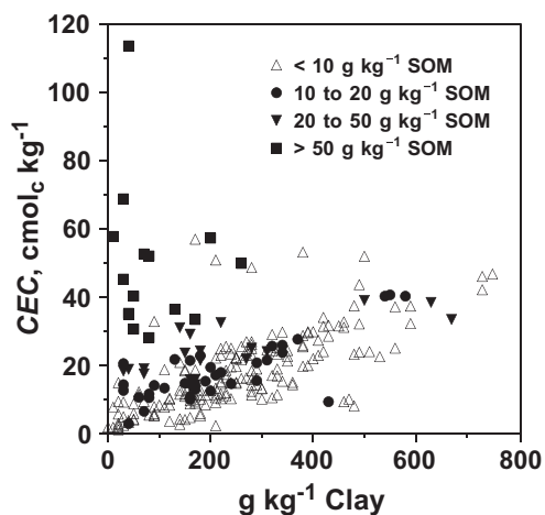
FIGURE 8.2 The cation exchange capacity ( CEC ) of 249 surface soil samples collected from around the U.S. as a function of soil clay content. The marker used to represent a particular data point indicates the soil organic matter (SOM) content of the soil sample. Data were obtained from Batjes (1995).
