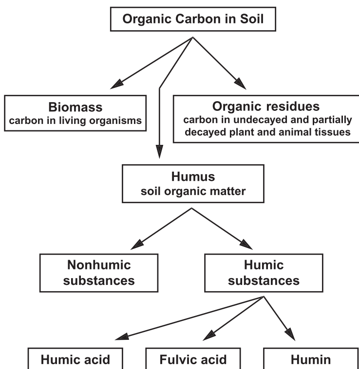
FIGURE 4.1 The pools of organic carbon in soil.
