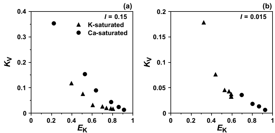
FIGURE 8.14 The Vanselow selectivity coefficient for KX-CaX 2 binary exchange in Loring (Oxyaquic Fragiudalf) soil as a function of E_K and ionic strength: (a) 0.15 and (b) 0.015.
