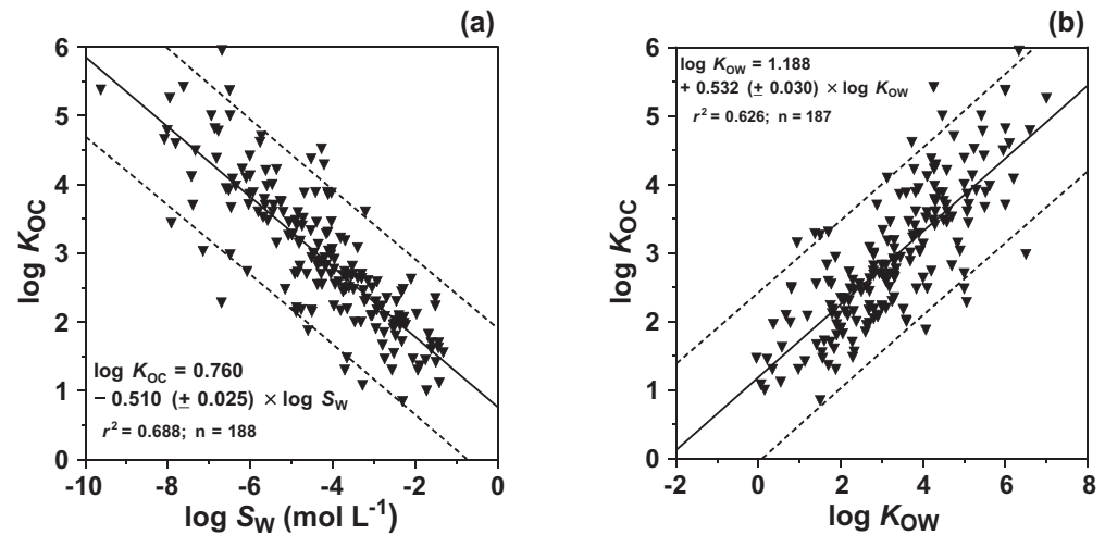
FIGURE 7.23 Relationship between soil organic carbon-normalized partition coefficient ( \log K_{oc} ) and water solubility ( \log S_w ) (a); and \log K_{oc} and octanol-water partition coefficient ( \log K_{ow} ) for organic pesticides (b). The solid lines represent the regression equation that appears on each diagram. The dashed lines represent the 95% confidence interval about the regression line. The data were obtained from numerous compilations and studies of individual compounds, and no attempt was made to group compounds according to similarities in physical-chemical properties.
