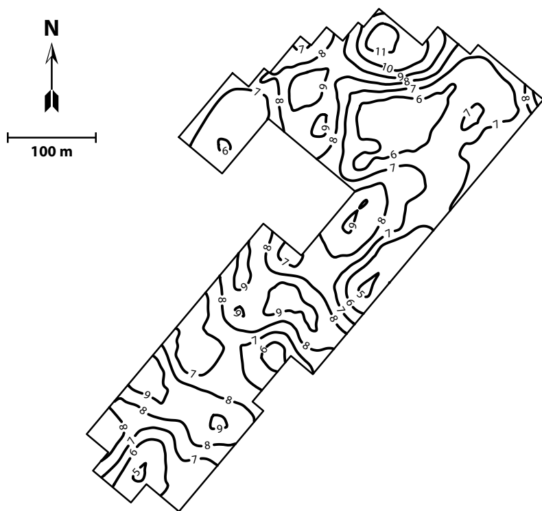
FIGURE 1.8 The spatial distribution of (a) effective cation exchange capacity ( ECEC , \text{cmol}_c \text{ kg}^{-1} ), (b) Mehlich-3-extractable Mn ( \text{mg kg}^{-1} ), and (c) soil organic carbon content ( \text{g kg}^{-1} ) in the surface soil (0–15 cm) on the 10.5 ha production cotton field located at the Milan Agricultural Experiment Station in Milan, TN.
