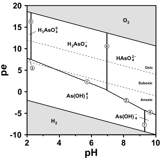
FIGURE 9.9 The redox speciation of As. The pe – pH diagram is specific to the following conditions: activities of the soluble As species are 10^{-6} ; activity of H_2O is unity; T = 25^\circ C ; and P = 0.101 MPa. The boundary lines are identified by number in Table 9.4 and the oxidic, suboxic, and anoxic pe – pH regions are illustrated.
