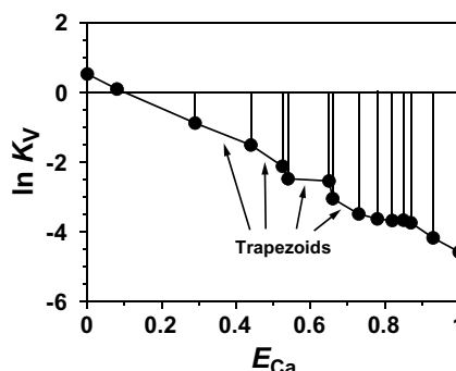
FIGURE 8.16 Plot of \ln K_V vs. E_{Ca} for the KX-CaX 2 binary exchange in Loring (Oxyaquic Fragiudalf) soil with an ionic strength of 0.15. The area bounded by the \ln K_V vs. E_{Ca} data and the \ln K_V = 0 axis is numerically equal to \ln K_{ex} and may be estimated using the trapezoid method (Table 8.6).
