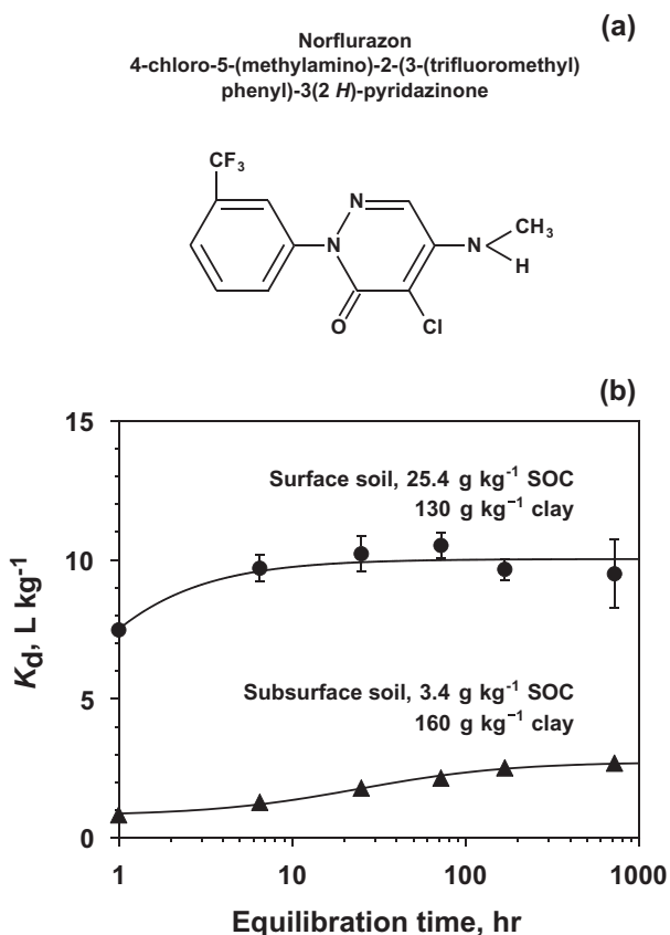
FIGURE 7.27 The structure of norflurazon (a), and the influence of equilibration time and soil organic carbon (SOC) and clay content (b) on norflurazon K_d values ( c_{in} = 170 \mu\text{g L}^{-1} ) and adsorption isotherms (c). The adsorption data were obtained by equilibrating 10-g samples of Lexington silt loam (Ultic Hapludalf) surface (0 to 8 cm) or subsurface (30 to 45 cm) soil, and 20 mL of 10 mM \text{CaCl}_2 solutions containing varied concentrations of the herbicide. The suspensions were equilibrated at 20 to 22°C. The error bars in (b) represent the range of K_d values obtained from replicate systems. When error bars are absent, the variation in K_d is smaller than the dimensions of the data point. The lines through the data in (c) represent Freundlich adsorption models obtained through nonlinear least-squares regression analysis. ( continued )
