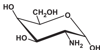
D-fucosamine
