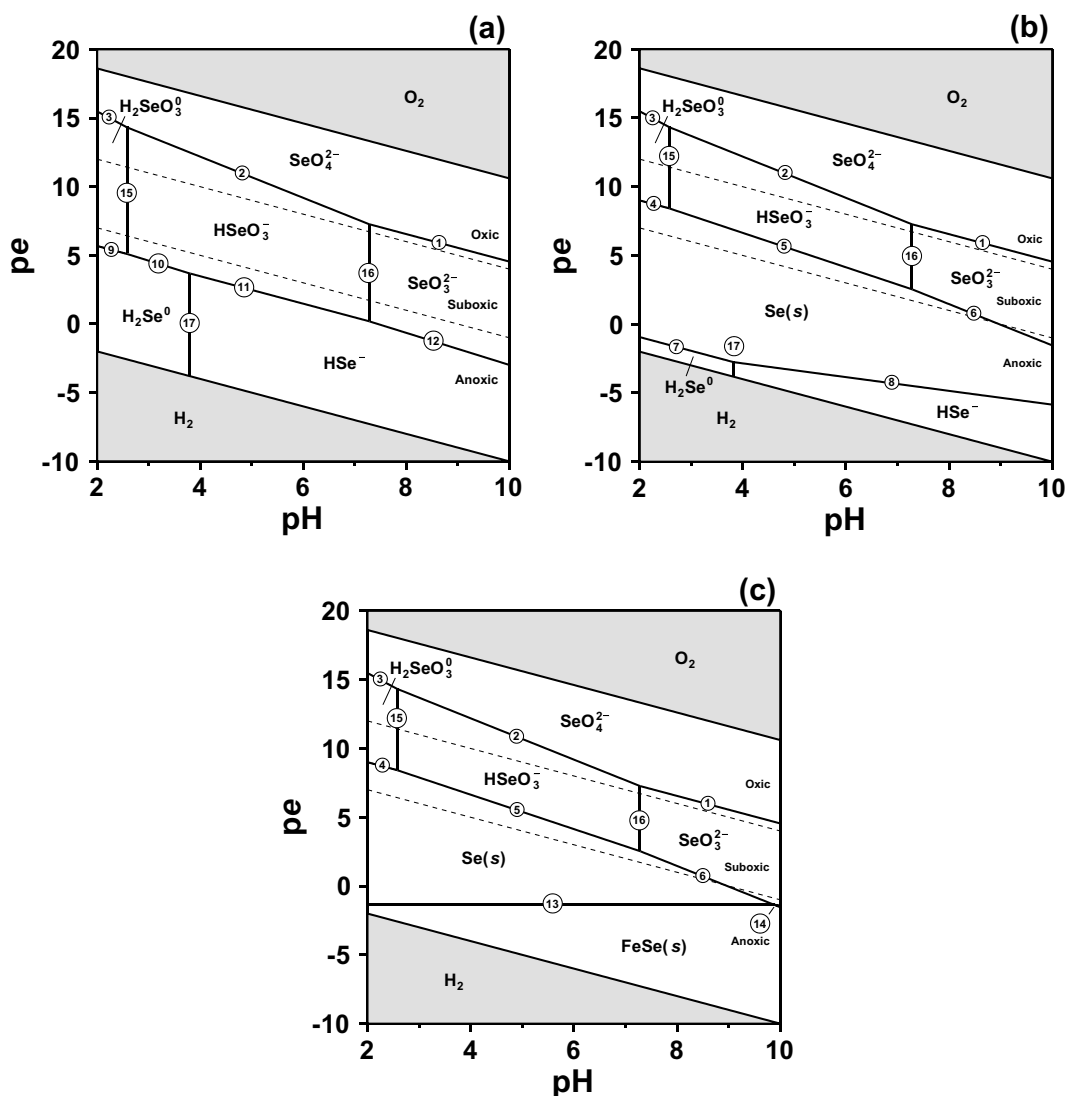
FIGURE 9.8 The redox speciation of Se. Diagram (a) considers only soluble Se species. Elemental Se is included in (b), and both elemental Se and FeSe(s) are included in (c). The pe–pH diagrams are specific for the following conditions: activities of the soluble Se species are 10^{-6} ; \text{Fe}^{2+} activity is 10^{-6} ; activities of \text{H}_2\text{O} and all solids are unity; T = 25^\circ\text{C} ; and P = 0.101 \text{ MPa} . The boundary lines are identified by number in Table 9.3, and the oxidic, suboxic, and anoxic pe–pH regions are illustrated.
